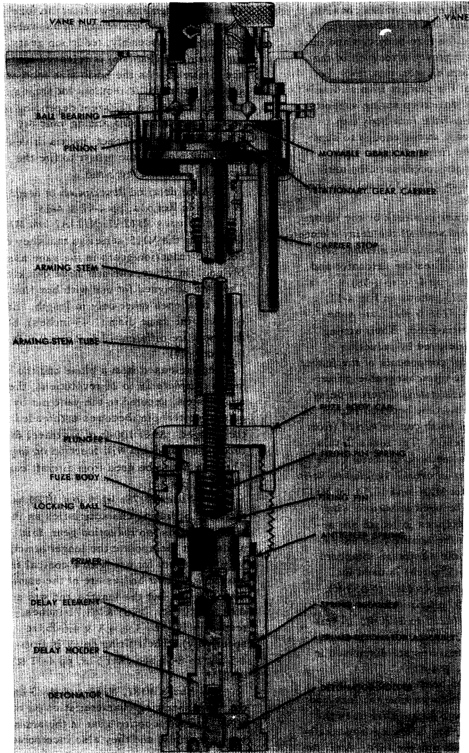
Fig 4-11 BOMB TAIL FUZE, M115
